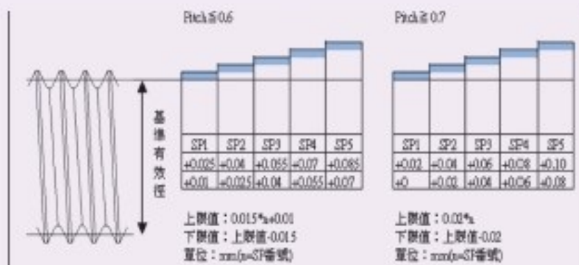
切削絲攻－SP精度 For Spial Taps - "SP" Accuracy
